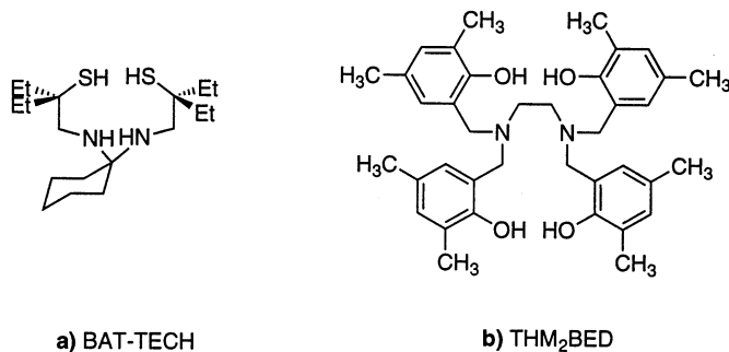
Fig. 8. (a) The N 2 S 2 ligand BAT-TECH whose Ga(III) complex showed significant myocardial uptake in an animal model. (b) The hexacoordinate N 2 O 4 ligand THM 2 BED which showed both heart and brain uptake in rats.
