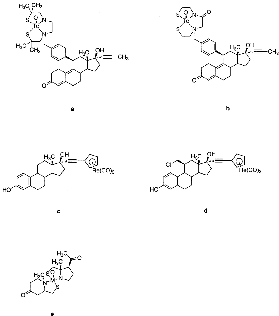
Fig. 27. Steroid based bioconjugates. Compounds (a) and (b) are \text{N}_2\text{S}_2 –progesterone conjugates for labeling with Tc and Re isotopes. Compounds (c) and (d) are organometallic–estrogen analogs. Compound (d) integrates the Tc or Re monooxo cation into the steroid structure.
