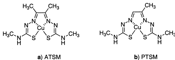
Fig. 21. Bis(thiosemicarbazone) Cu(II) complexes utilized for imaging hypoxic tissue (a) and for perfusion (b).
