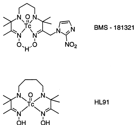
Fig. 3. ^{99m}\text{Tc} -labeled hypoxia imaging agents.
